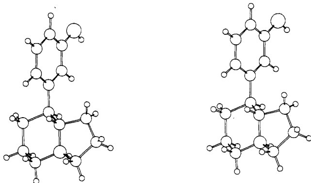
Figure 5. Stereoscopic view of the X-ray structure of (8 S )-19e-HCl salt.
