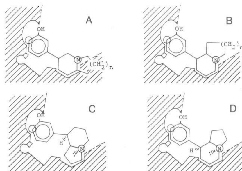
Figure 4. Fittings of (3-hydroxyphenyl)indolizidines and -quinolizidines in a DA receptor model proposed by H. Wikström. 5,6 A, fit of 17e and 18e; B, fit of 19e and 20e; C, fit of (8R)-19e; D, fit of (8S)-19e.
